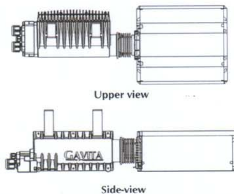
GAN Electronic 600W 230V with Ecomax HR 96 Reflector
