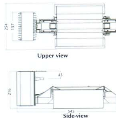
GAN Electronic 600W / 750W / 1000W 400V with Ecomax HR 96 Reflector
